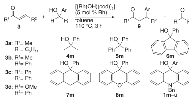
Scheme 3. Rhodium-catalyzed conjugate arylation of α,β-unsaturated carbonyl compounds through β-aryl elimination.
